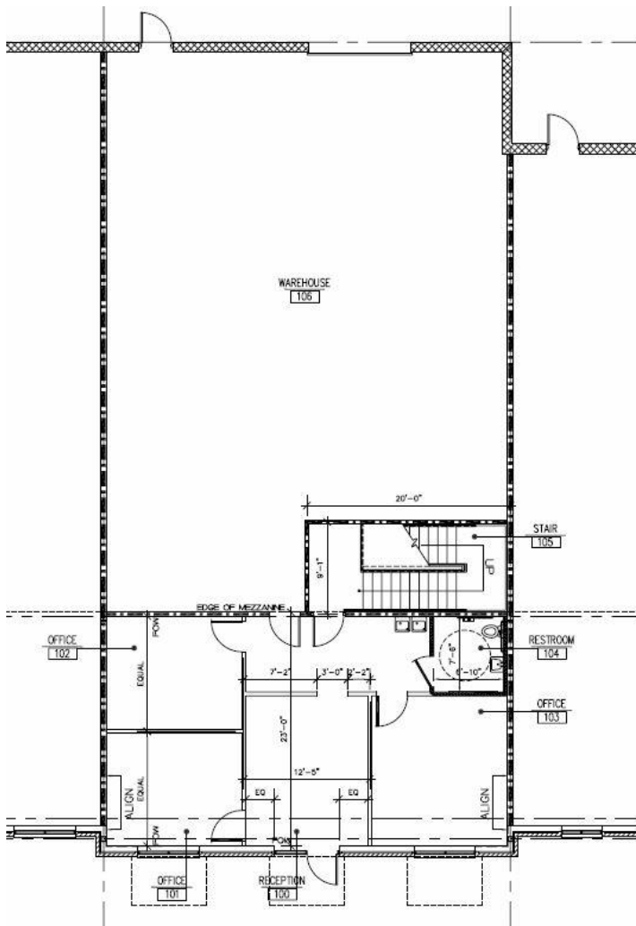
1 DIMENSION PLAN - 1ST FL 1D-1.0 SCALE: 1/8" = 1'-0"
