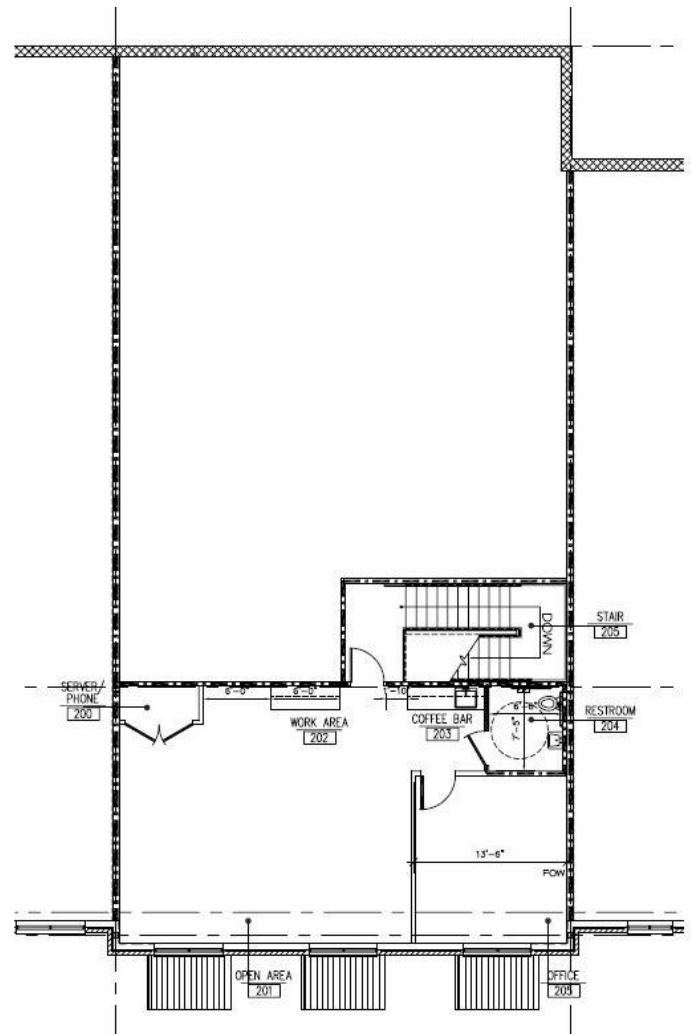
2 DIMENSION PLAN - 2ND FL 1D-1.0 SCALE: 1/8" = 1'-0"
