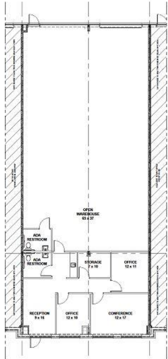
UNIT 300 - FLOOR PLAN
